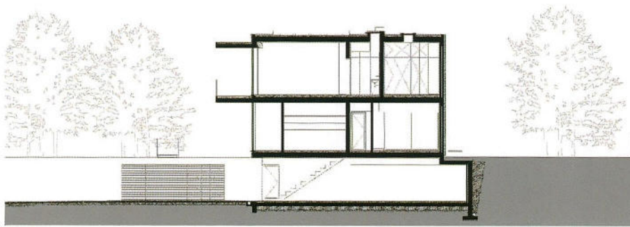
SECTION 1
